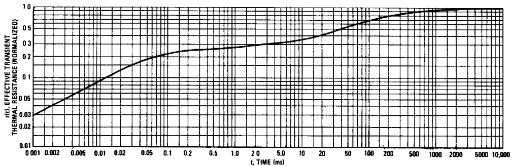
FIGURE 3 - THERMAL RESPONSE
